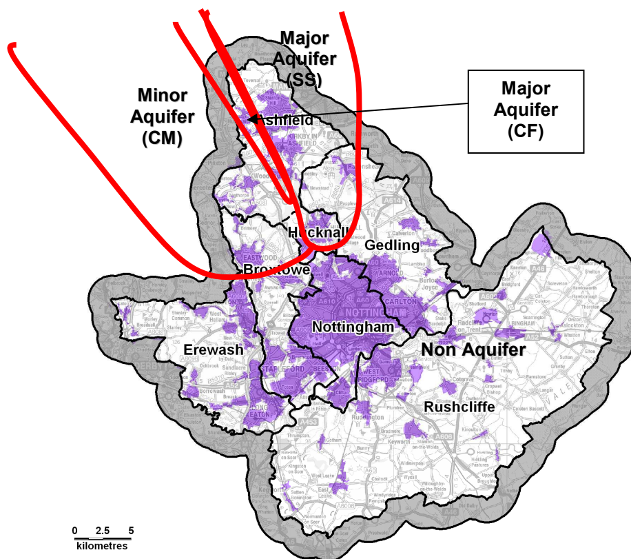
Figure 5-1: Simplified Location of Main Aquifers around Greater Nottingham Key – CM Coal Measures, CF Cadeby Formation, SS Sherwood Sandstone
