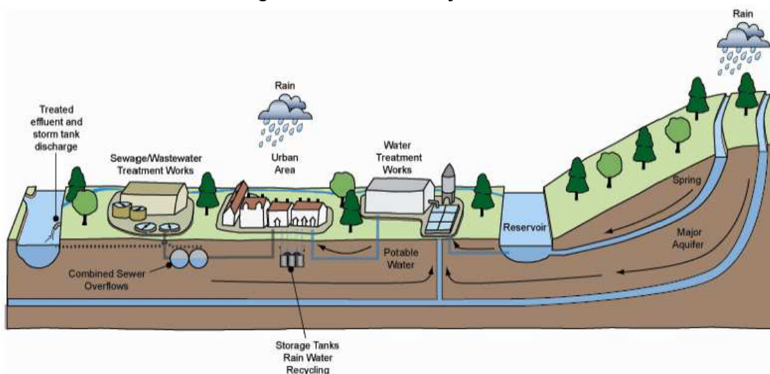
Figure 3-1: The Water Cycle
